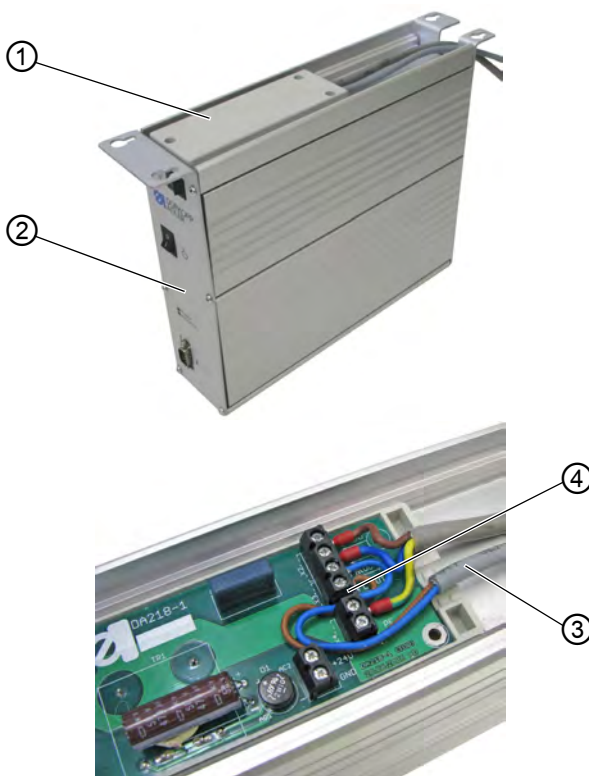
Image 62: Raccorder la lampe de couture (1)
