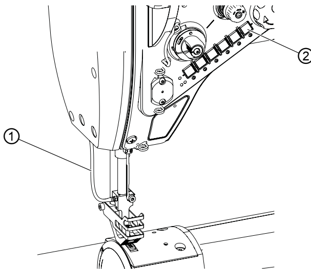
Fig. 38: Needle cooling
