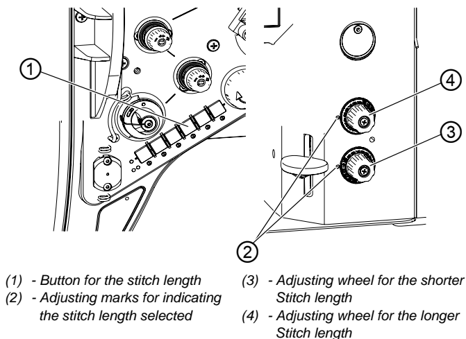
Fig. 31: Sewing with 2 stitch lengths
