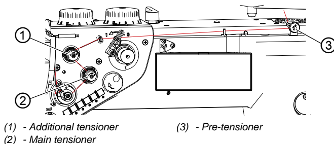
Fig. 17: Setting the needle thread tension
