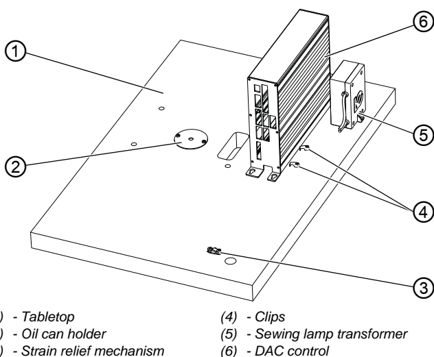
Fig. 51: Machines with long arm
