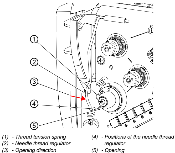
Fig. 20: Setting the needle thread regulator
