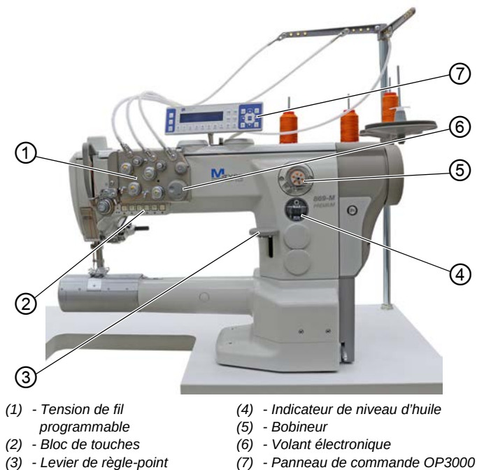
Image 1: Composants de la machine
