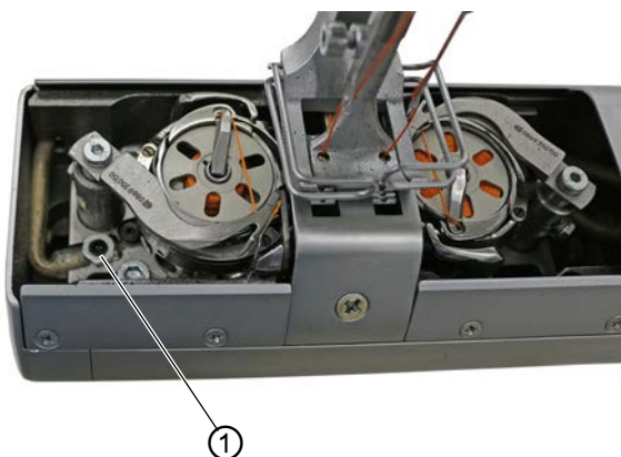
Image 55: Lubrifier le crochet
