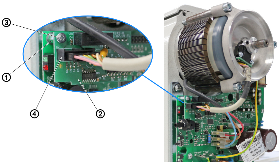
Abb. 2: Assembling and connecting the additional PCB (2)
