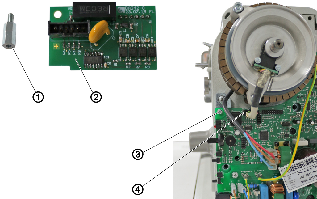
Abb. 1: Assembling and connecting the additional PCB (1)
