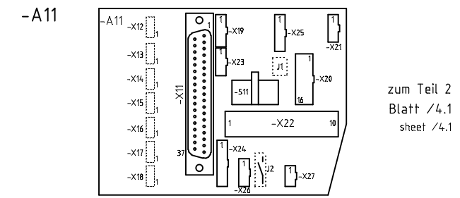
PCB 9850 867000 distribution board
