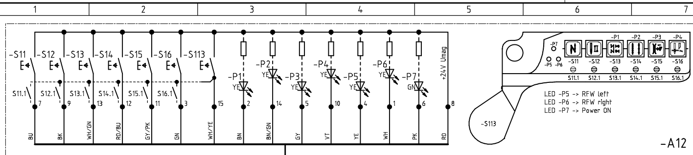
Keypad 9880 670001 or Keypad 9880 680001 (only 670) (only 680)
