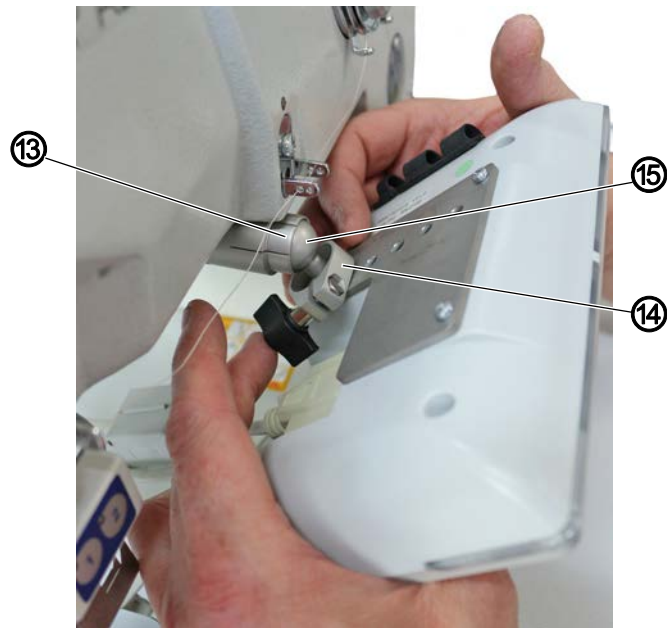
Abb. 15: Bedienfeld Commander Basic/Pro montieren (7)
