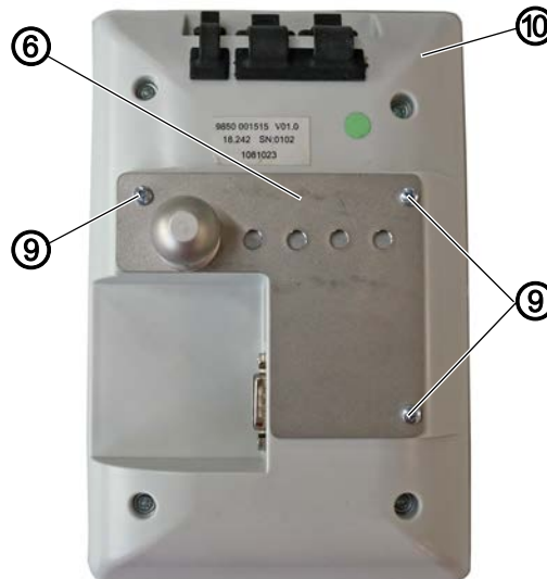
Abb. 13: Bedienfeld Commander Basic/Pro montieren (5)
