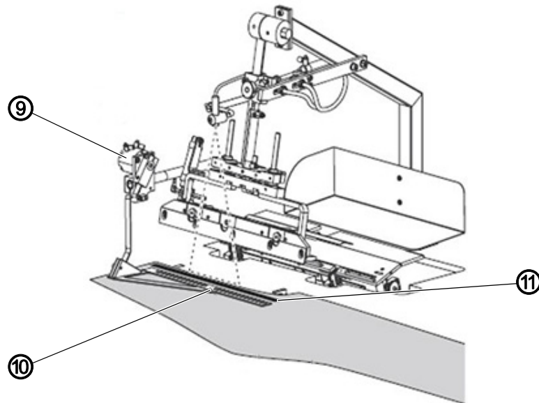
Fig. 11: Sewing the right fly piece onto the right trouser component (2), lining up the right fly piece
