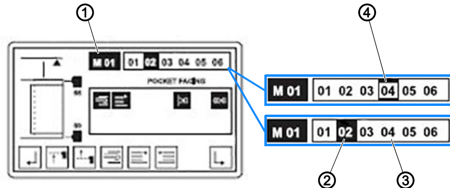
Fig. 22: Selecting a seam program
