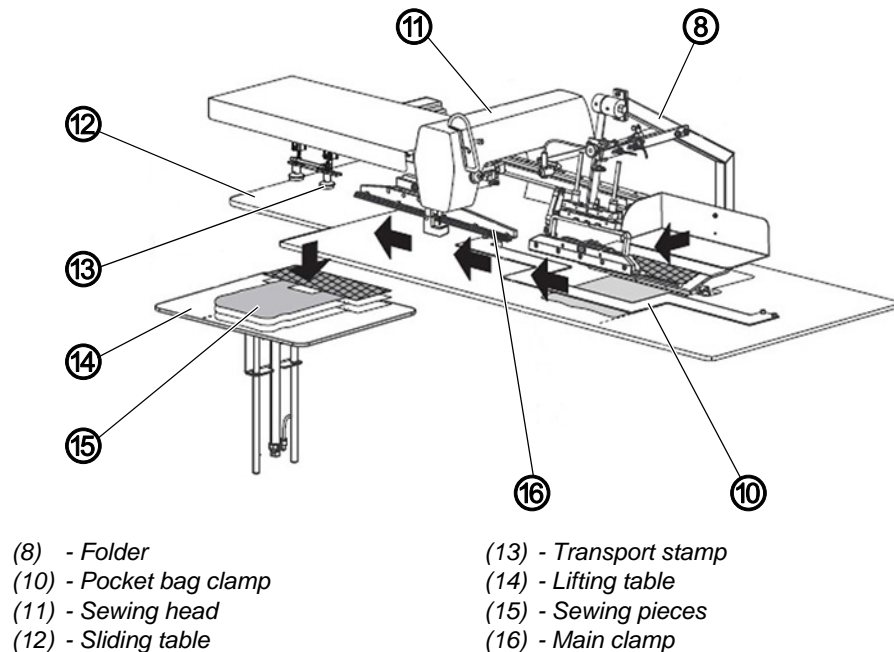
Fig. 6: Sewing on pocket facing (4), transport and sewing
