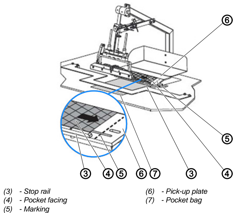
Fig. 4: Sewing on pocket facing (2), positioning and aligning
