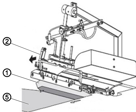
Fig. 17: Lapping the right wing pocket to the right trouser component (2), sewing the right wing pocket to the trouser component
