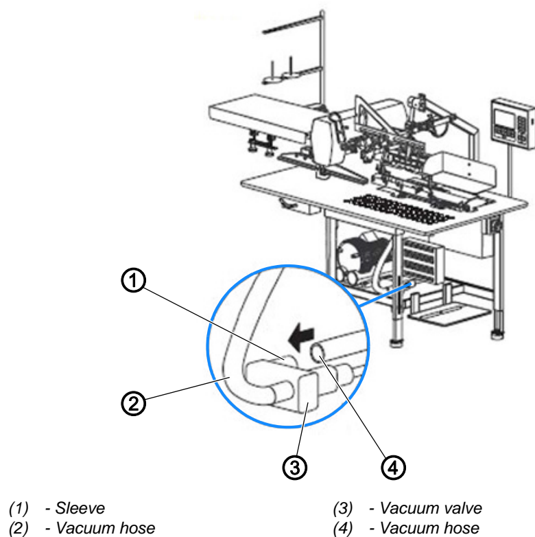
Fig. 29: Connecting the vacuum device
