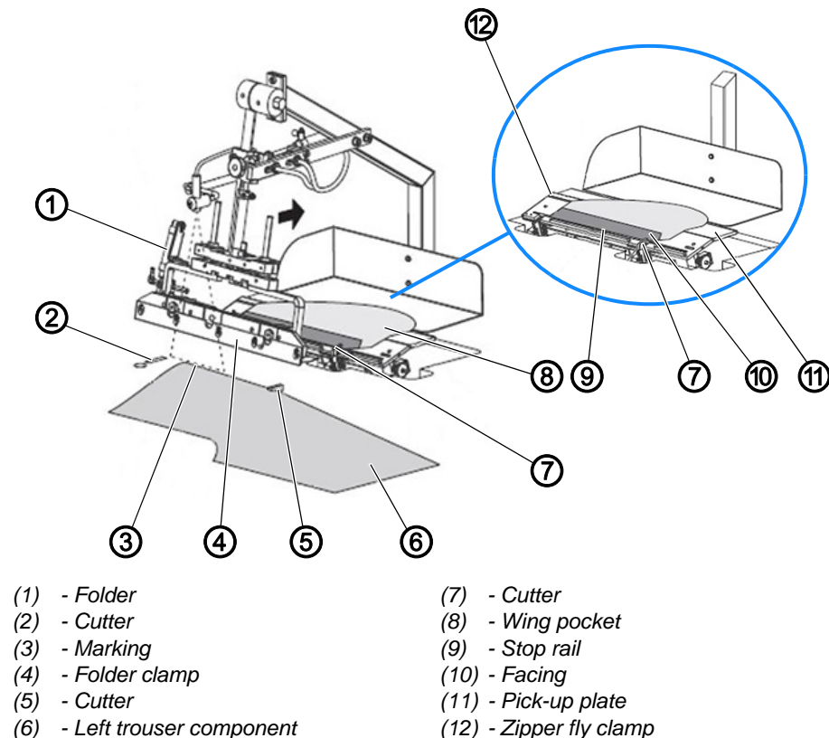
Fig. 13: Lapping the left wing pocket to the left trouser component (1), lining up the left wing pocket and the trouser component
