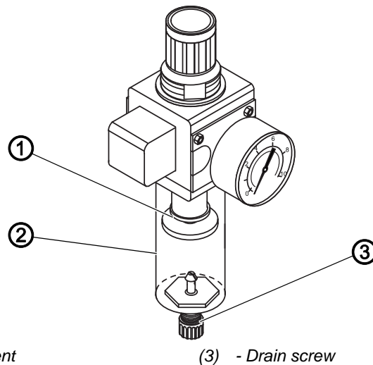
Fig. 25: Cleaning the filter element
