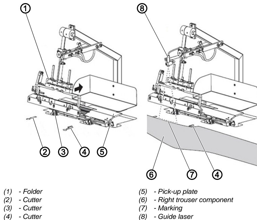
Fig. 10: Sewing the right fly piece onto the right trouser component (1), lining up the right trouser component
